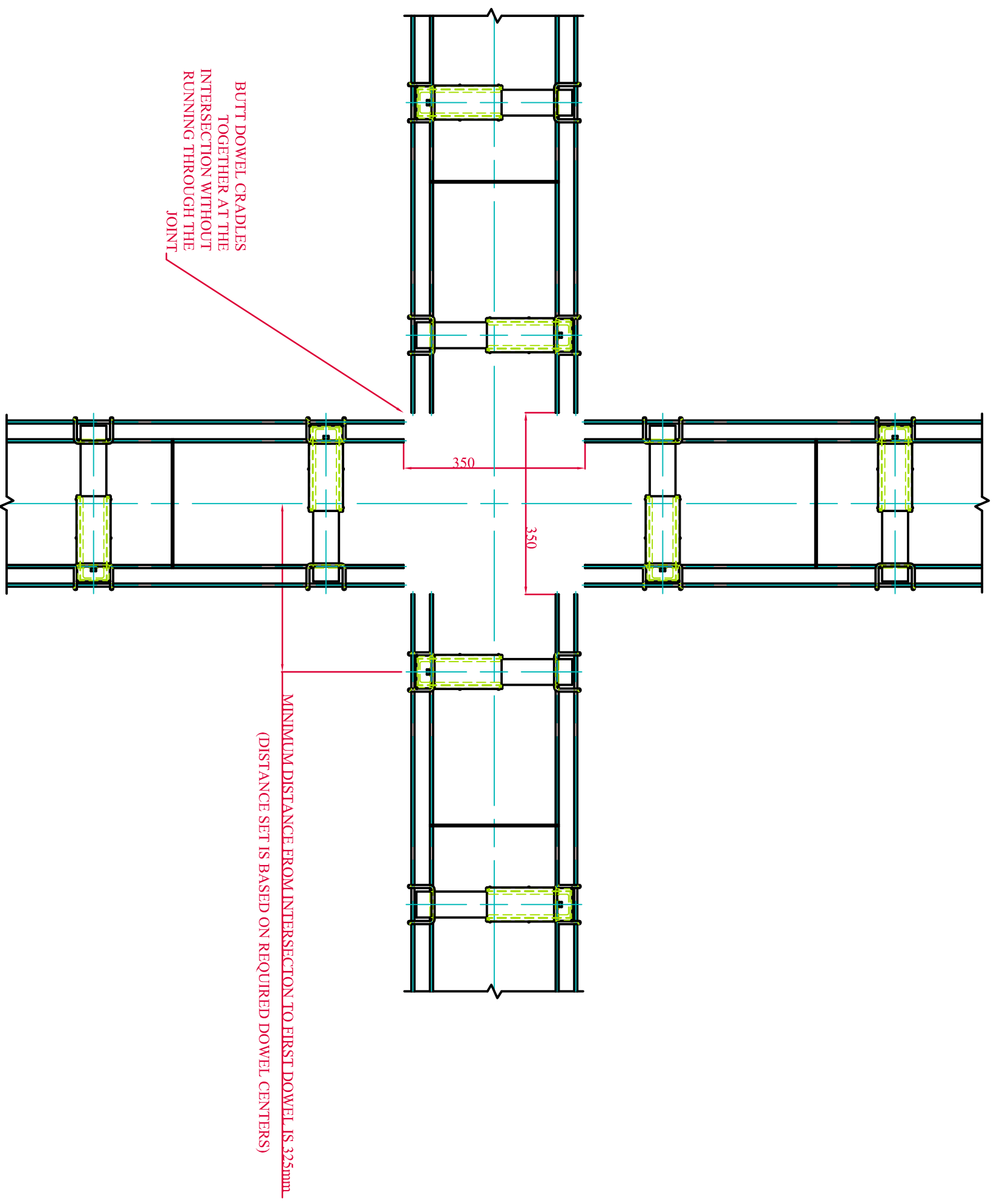
PLAN VIEW AT 4-WAY INTERSECTION
