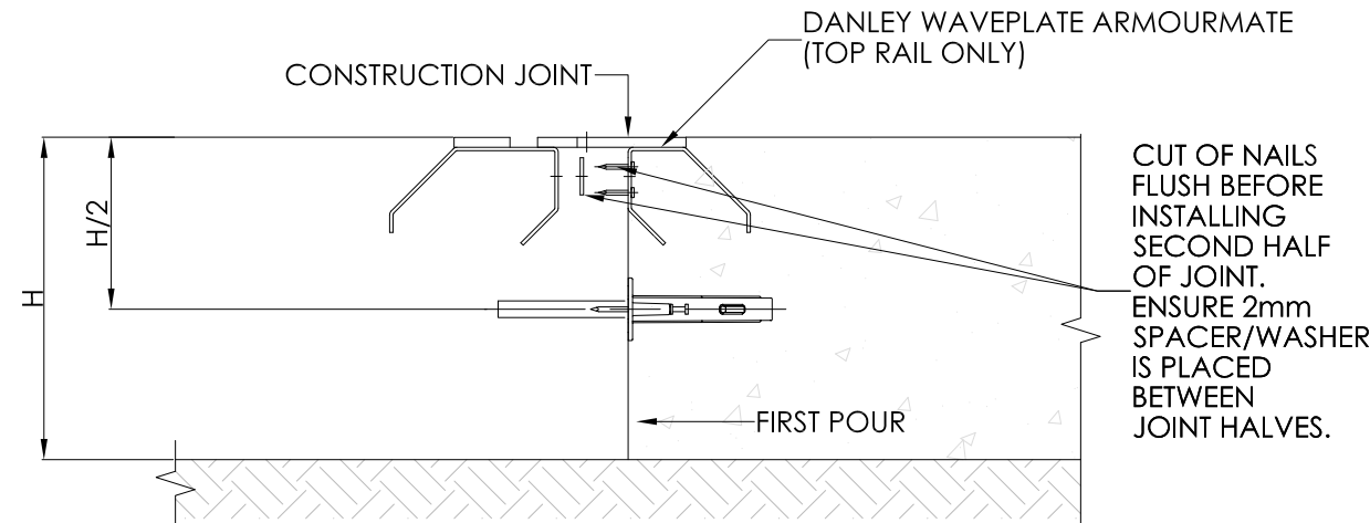
STEP 2 - ARMoured DOWEL JOINT (A.D.J.) SCALE: 1:5
