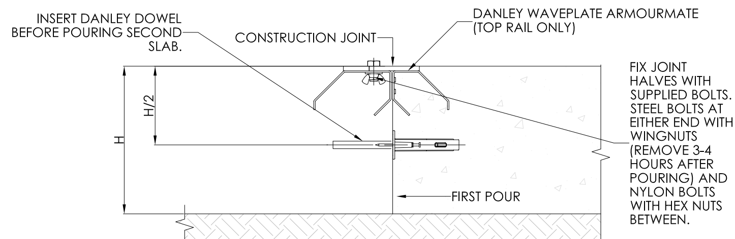
STEP 3 - ARMoured DOWEL JOINT (A.D.J.) SCALE: 1:5
