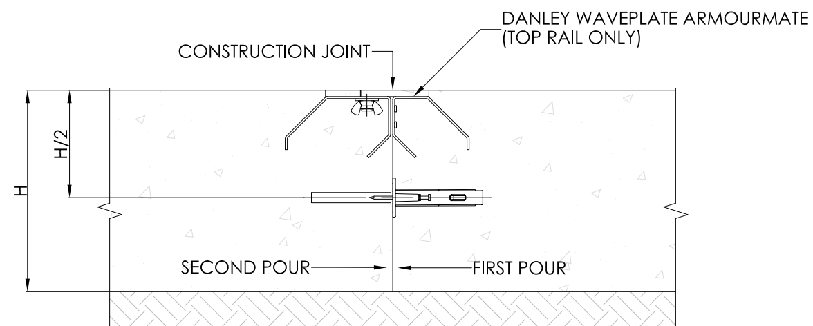
STEP 4 - ARMoured DOWEL JOINT (A.D.J.) SCALE: 1:5
