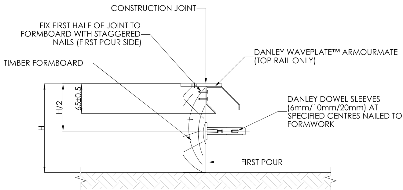
STEP 1 - ARMoured DOWEL JOINT (A.D.J.) SCALE: 1:5
