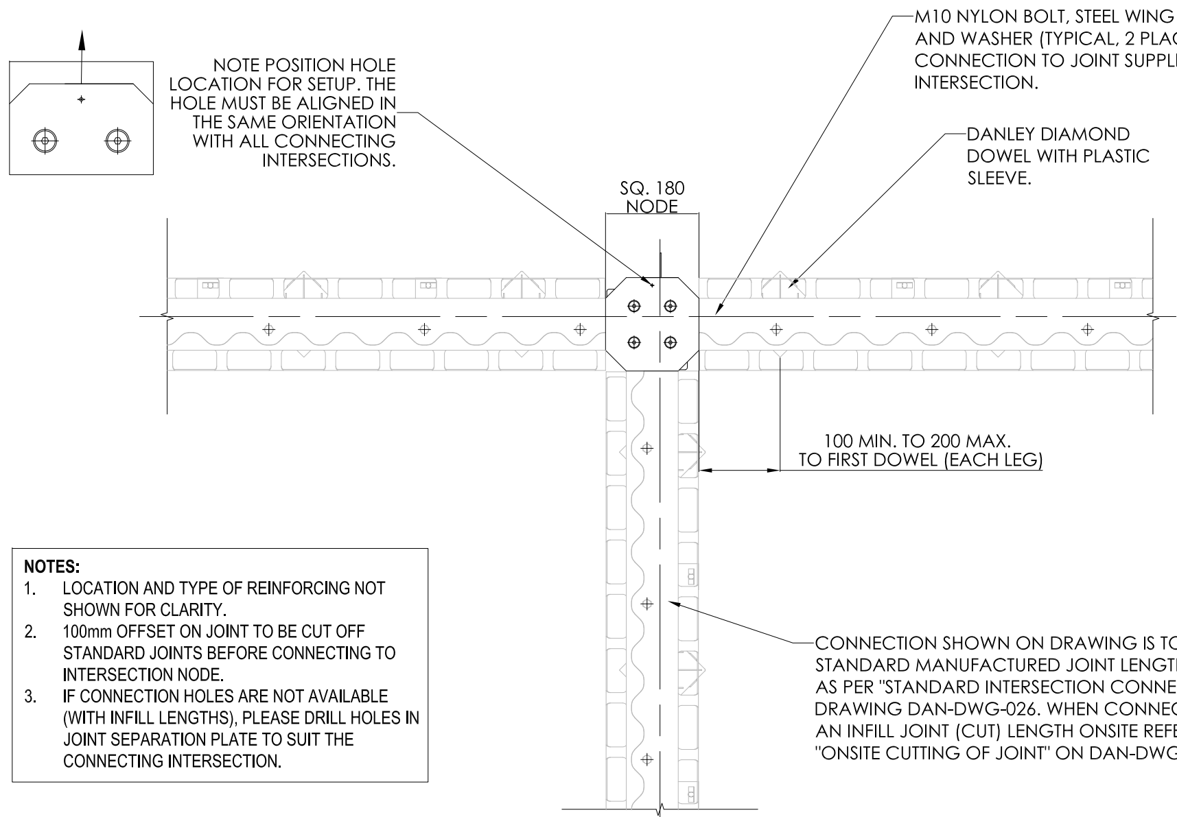
WAVEPALTE ARMOUMATE AT 3-WAY INTERSECTION SCALE: 1:10
