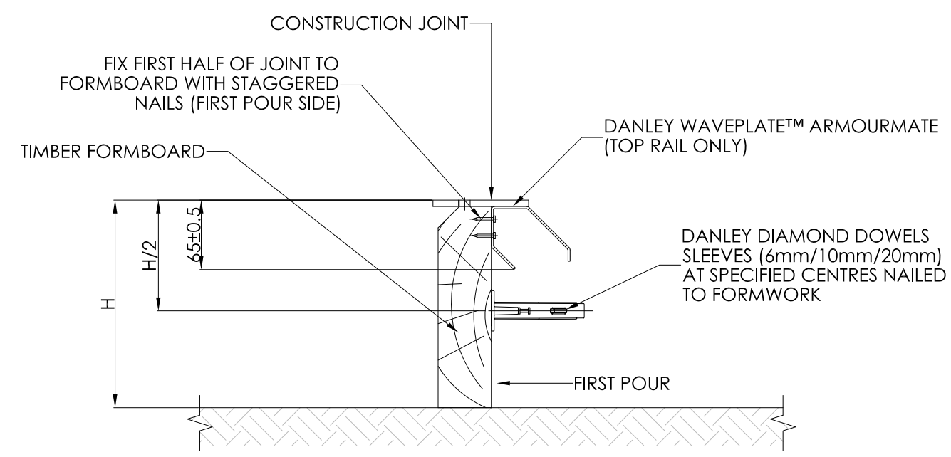
STEP 1 - ARMoured DOWEL JOINT (A.D.J.) SCALE: 1:5
