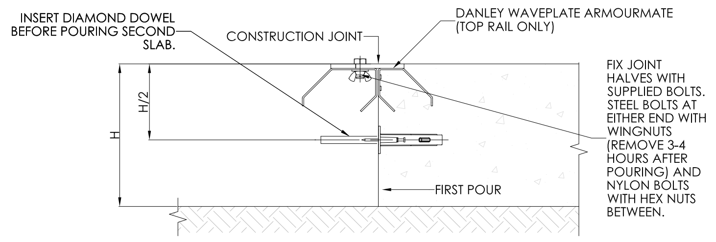
STEP 3 - ARMoured DOWEL JOINT (A.D.J.) SCALE: 1:5
