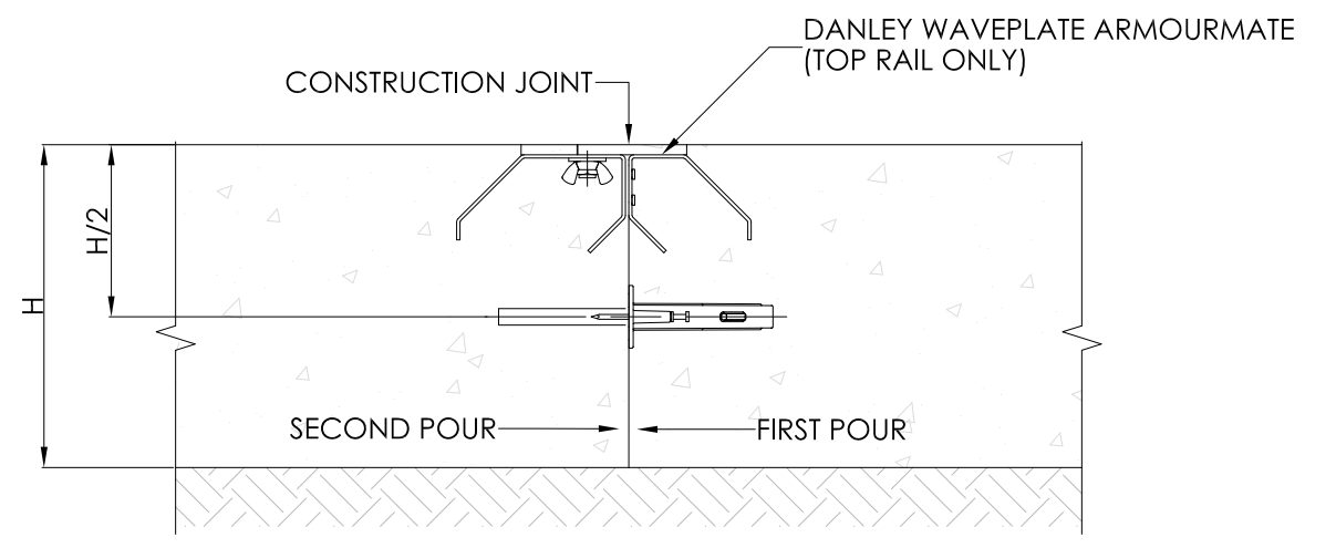
STEP 4 - ARMoured DOWEL JOINT (A.D.J.) SCALE: 1:5
