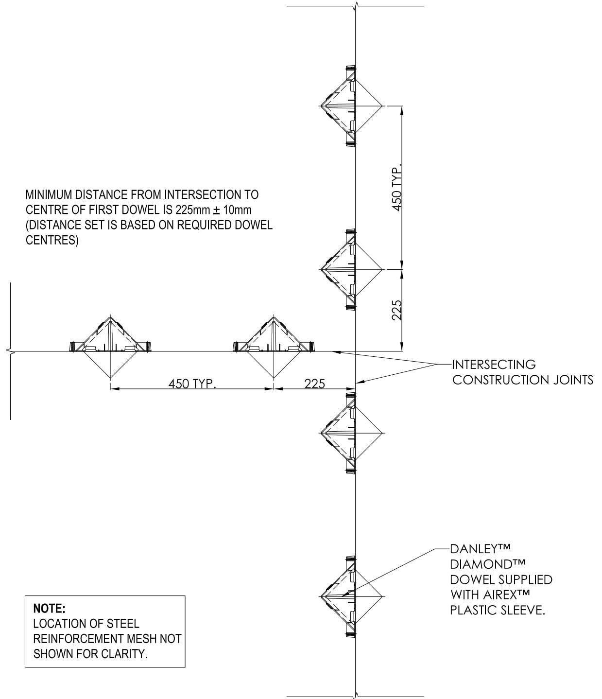
DIAMOND™ DOWEL AIREX™ AT 3-WAY INTERSECTION SCALE: 1:10
