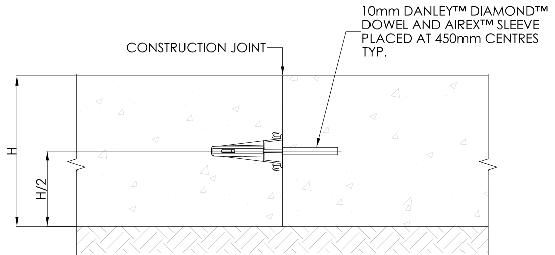
PLATE DOWEL JOINT (P.D.J.) SCALE: 1:5
