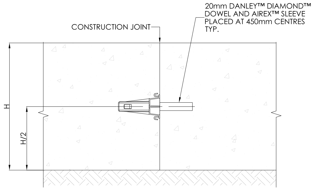
PLATE DOWEL JOINT (P.D.J.) SCALE: 1:5
