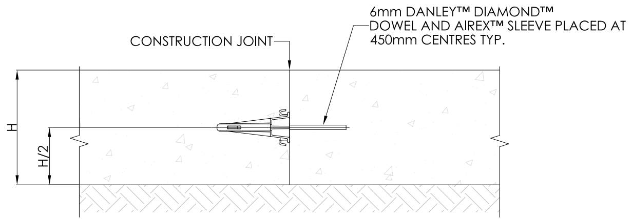
PLATE DOWEL JOINT (P.D.J.) SCALE: 1:5
