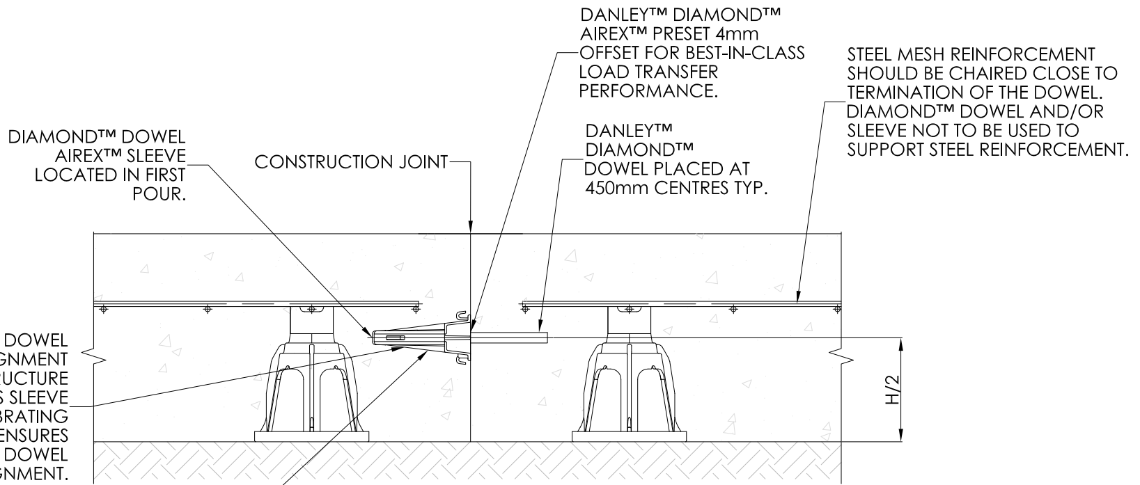
PLATE DOWEL JOINT (P.D.J.) SCALE: 1:5
